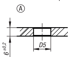
Push-in ball lock pin
