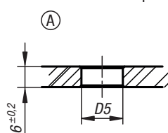
Push-in ball lock pin
