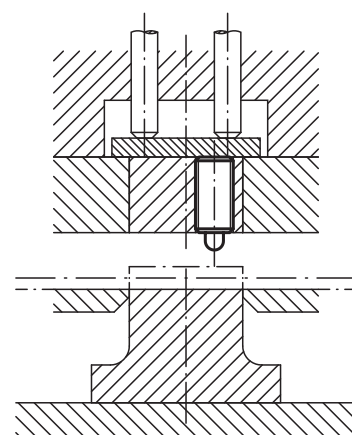
Spring plunger sectional view
