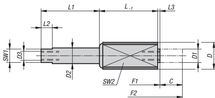
push-pull plunger
