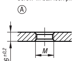
Screw-in ball lock pin
