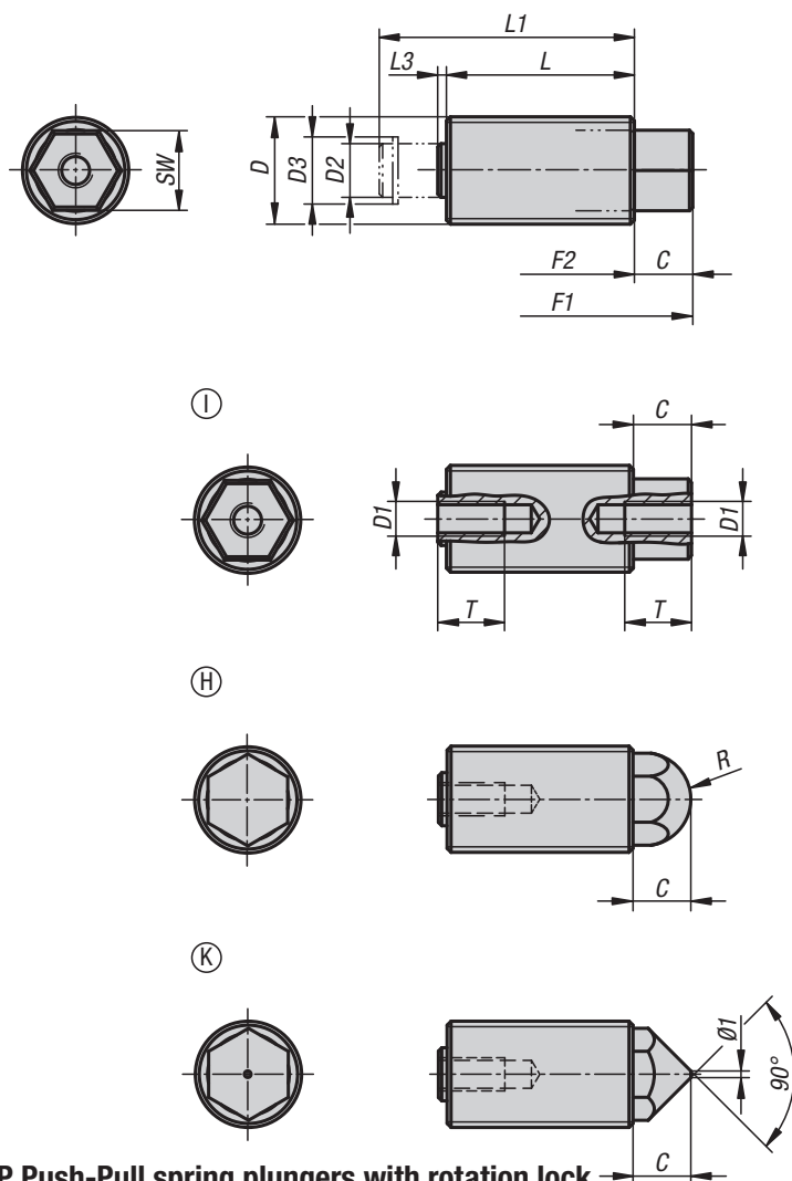
KIPP Push-Pull spring plungers with rotation lock
