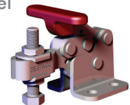
307-USS Flanged Base U-Bar, Stainless Steel
