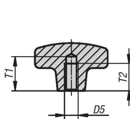
Style E tapped blind hole
