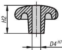
Style B reamed through hole
