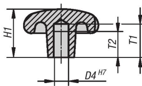
Style C reamed blind hole
