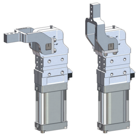
82M-3E03... U-Arm, 90° 82M-3E03... U-Arm, 180°
