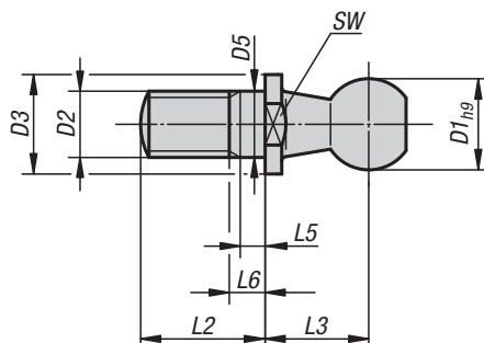
Form C with thread and flats
