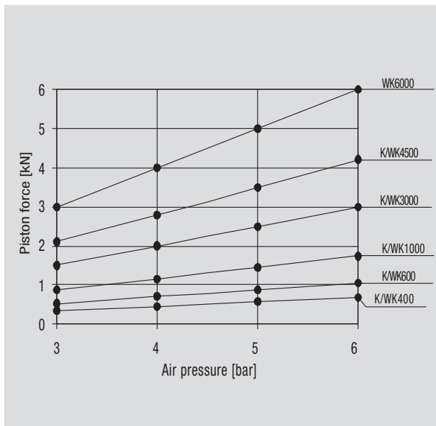
Force within forward stroke
