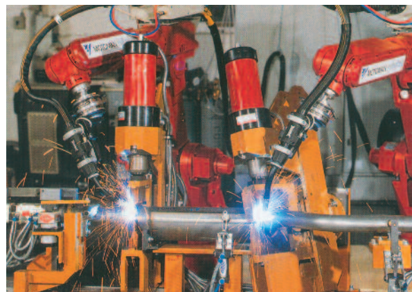
Welding fixture for exhaust components
