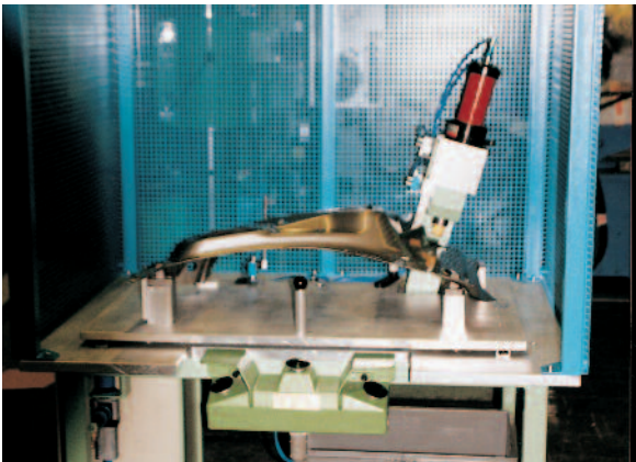
Device for holes Ø 8 in sheet metal
