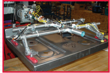
Stove Top Transfer with Round Tooling
