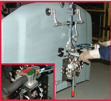
Manual Assesst with Round Tooling
