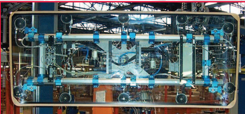
Glass Handling with BodyBuilder™ and Vacuum Cups
