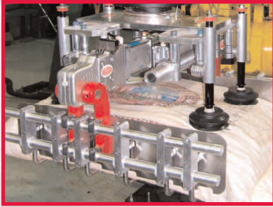
Bag Lifting and Palletizing Tool
