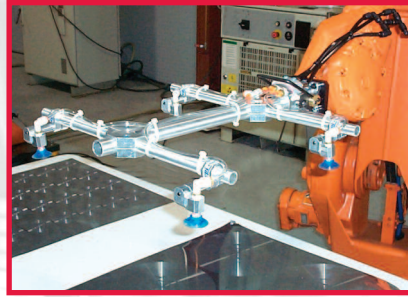
Sheet Metal lifting with Round Tooling
