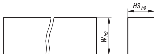
Installation dimensions counterpart square bar
