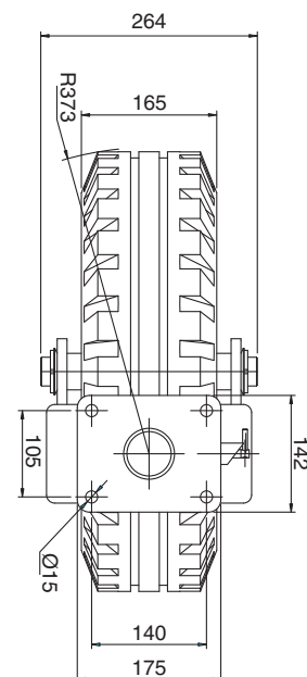
WHEEL FACE BRAKE OPTION - SUFFIX 'WFB'
