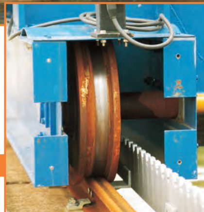
Bridge scraper for rectangular settlement tank
