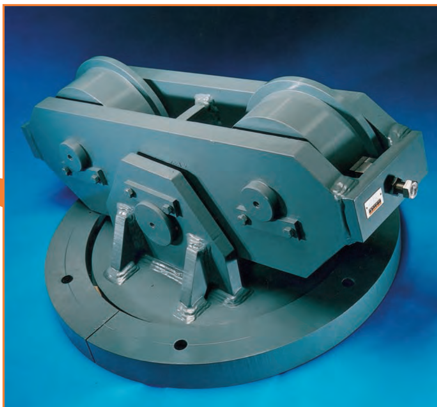
Pivoting castor with swivel head fitted with two EN24T single flange rail wheels complete with wheel brakes. Tread diameter 280mm. Tread width 87.5mm. Tread flame hardened. Maximum load rating per castor 45000Kg.
